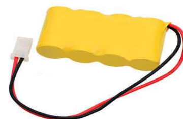
ES1.8-4.8 NICAD (4.8V 1.8Ah W/Plug)
