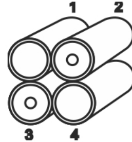
ES0.8A-4.8W-NICAD (4.8V 0.8Ah Wire Lead)
